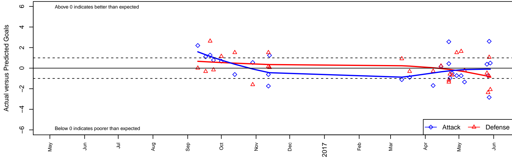
FC Nova Gold B02 Dots are actual minus expected GF (blue circles) and GA (red triangles). Blue line is smoothed change in attack strength. Red is smoothed change in defense strength.
